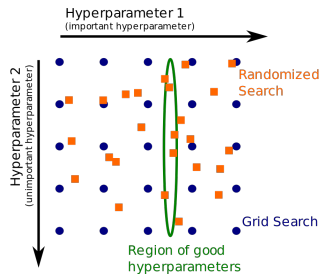
Figure 10: Grid Search vs. Random Search in Hyperparameter Tuning.
